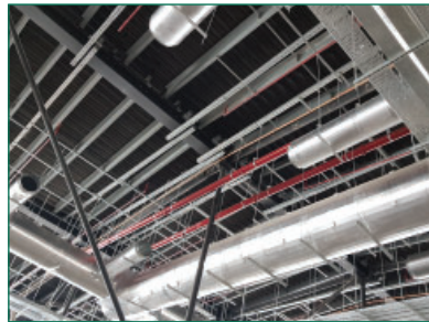
Secondary Steel Support
